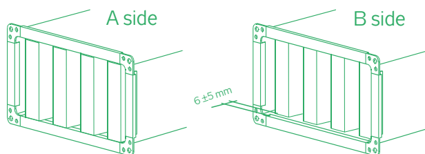
FIGURE 3 – ALIGNMENT OF ATTENUATORS, WHEN CONNECTED TOGETHER
