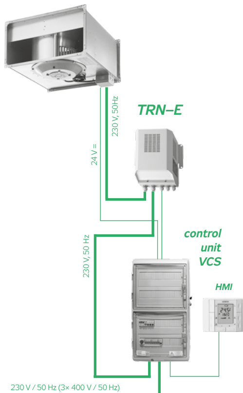
FIGURE 10 – FAN CONNECTION
