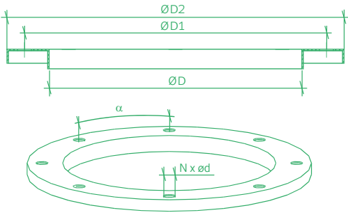
FIGURE 1 – DIMENSIONAL RANGE
