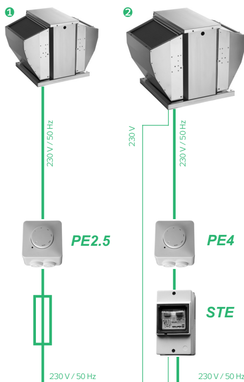
FIGURE 7 – FAN CONNECTION
