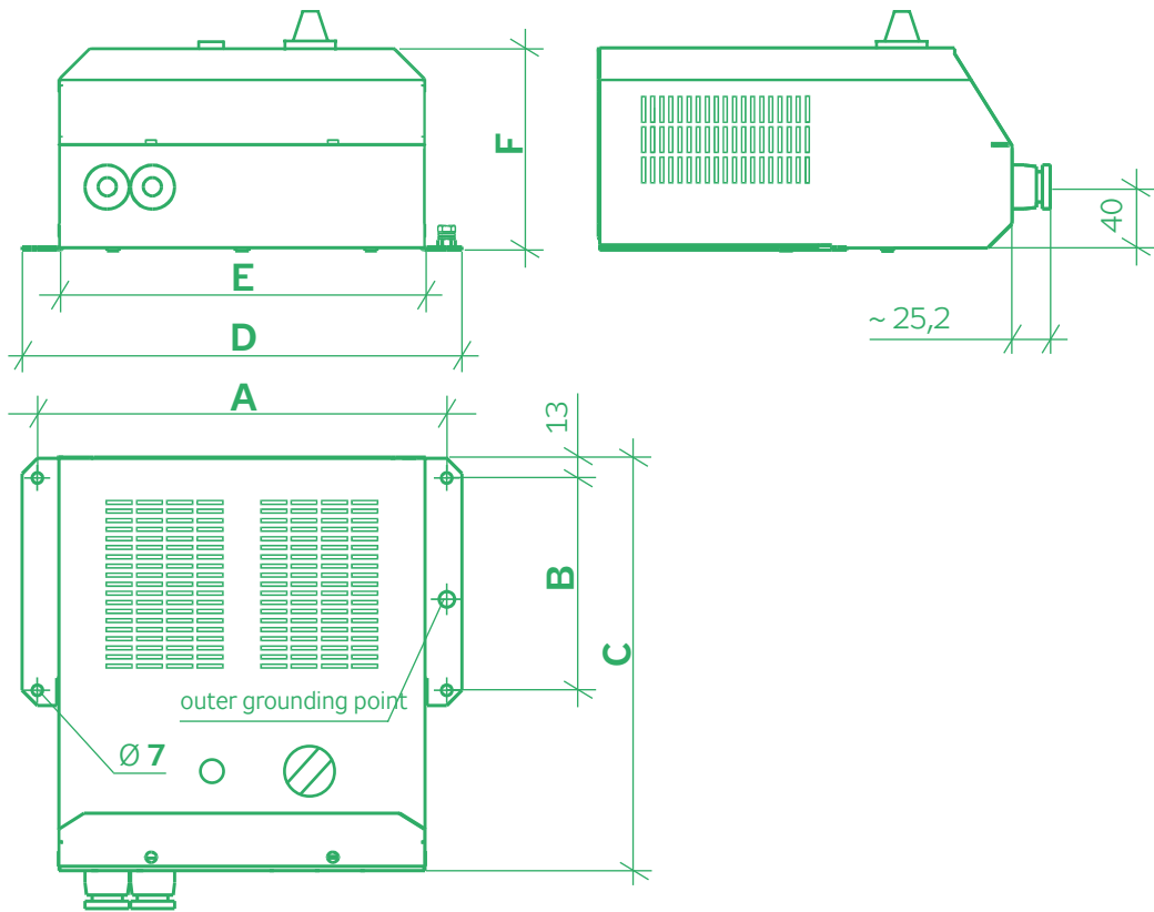
FIGURE 32 – CONTROLLER DIMENSIONS
