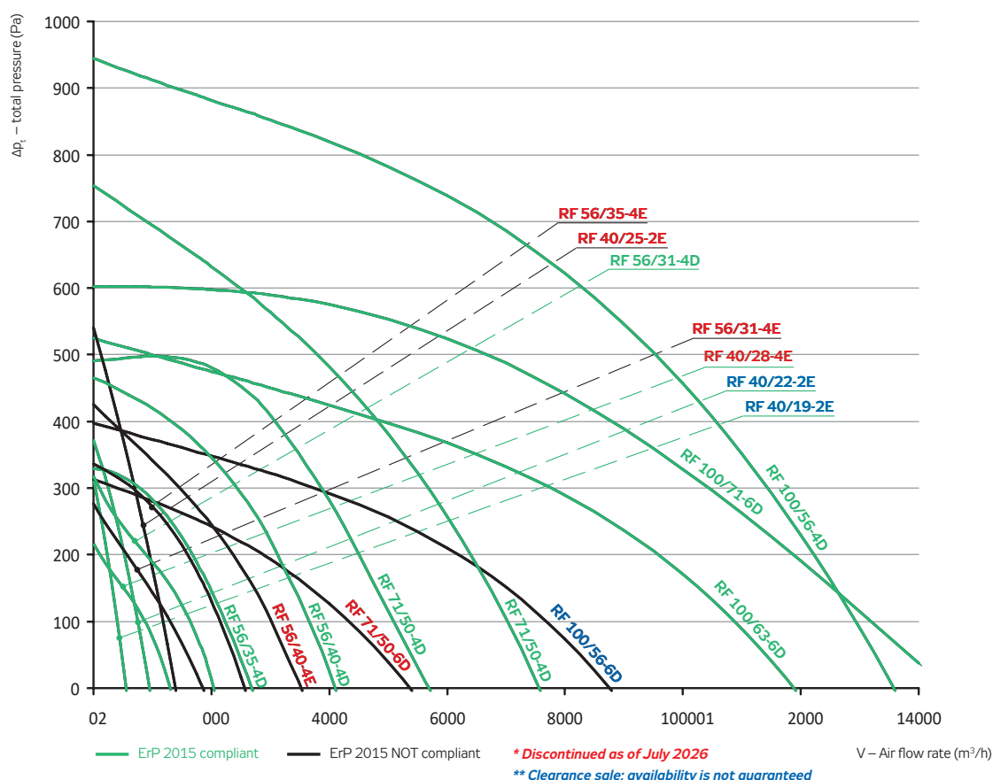
GRAPH 2 – RF FAN CHARACTERISTICS QUICK SELECTION
