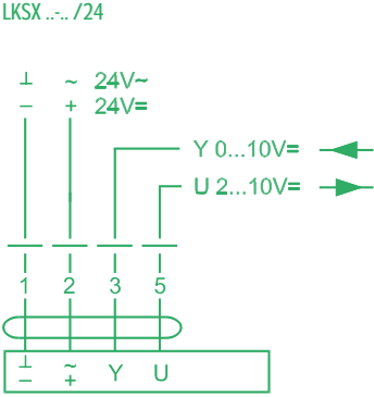
FIGURE 4 – DAMPER ACTUATOR WIRING DIAGRAM
