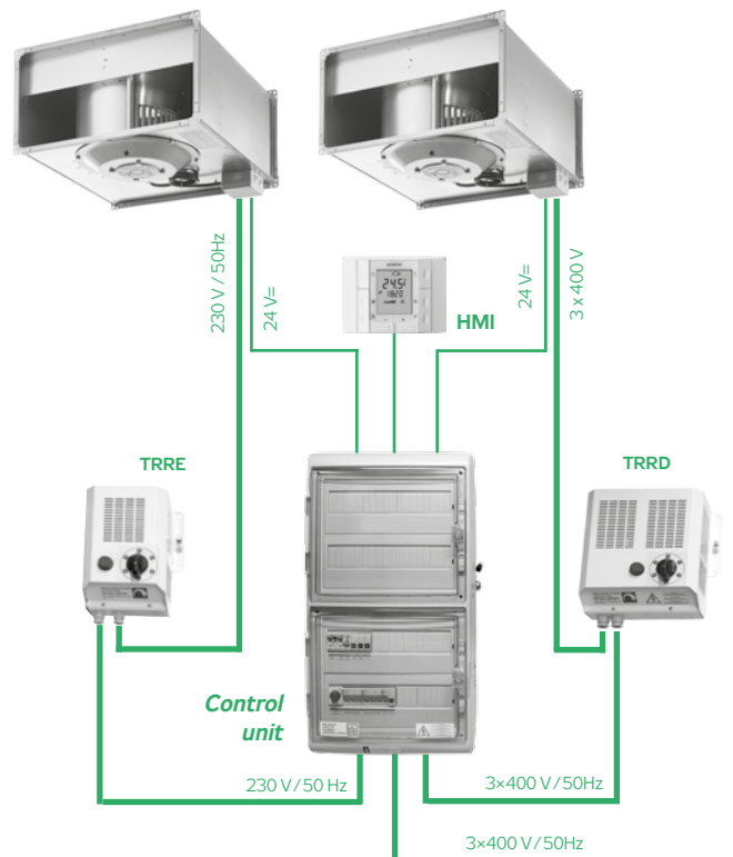
FIGURE 36 – CONTROLLER CONNECTION
