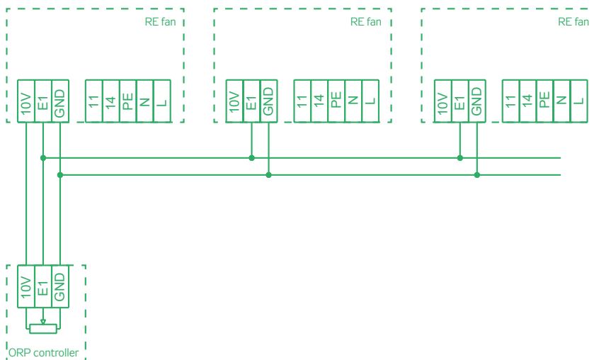
FIGURE 43 – ORP CONTROLLER CONNECTION TO MULTIPLE RE FANS
