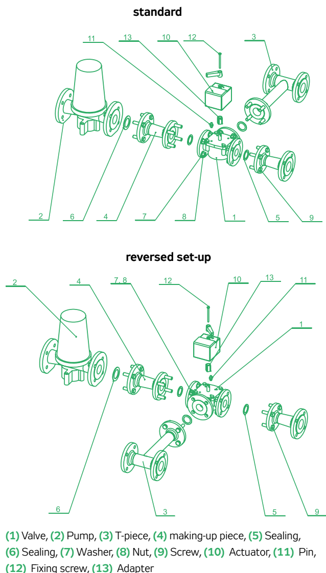
FIGURE 7 – EXPLODED VIEW OF THE MIXING SET
