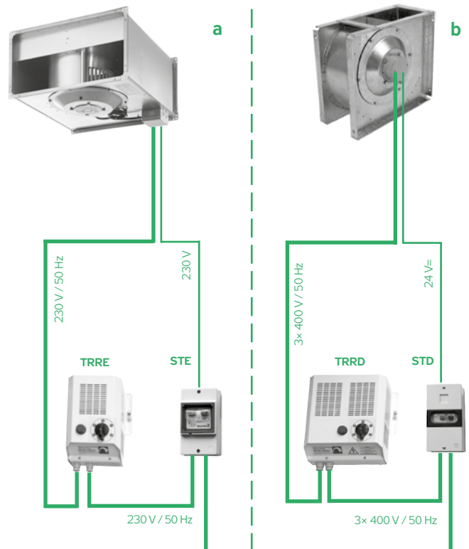
FIGURE 35 – CONTROLLER CONNECTION
