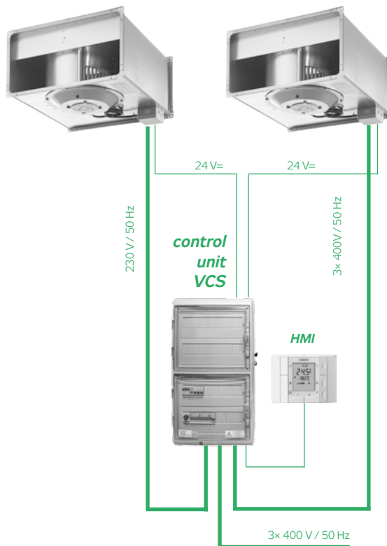
FIGURE 9 – FAN CONNECTION
