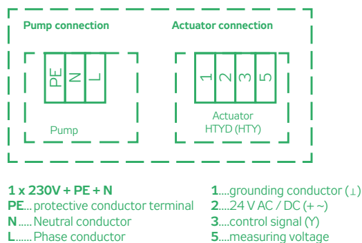
FIGURE 8 – MIXING SET WIRING DIAGRAM
