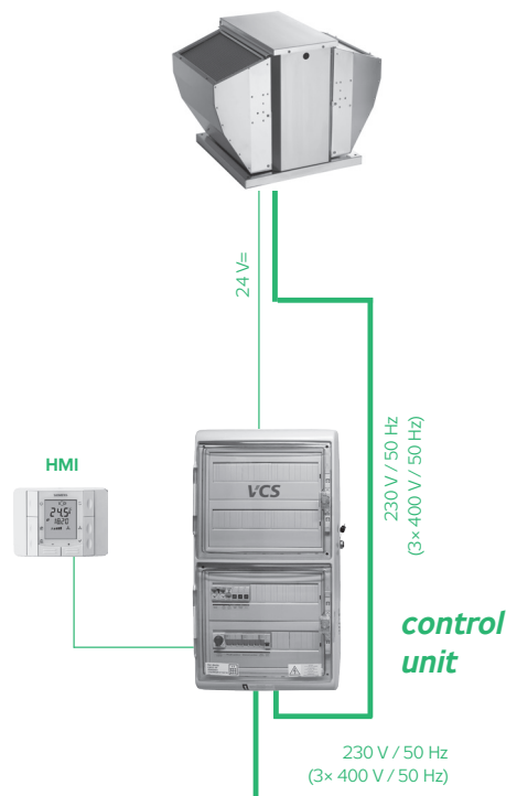
FIGURE 10 – FAN CONNECTION
