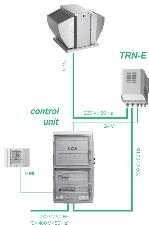
FIGURE 11 – FAN CONNECTION
