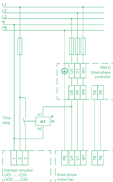
FIGURE 20 – LKS, LKSF DAMPERS WIRING SCHEME
