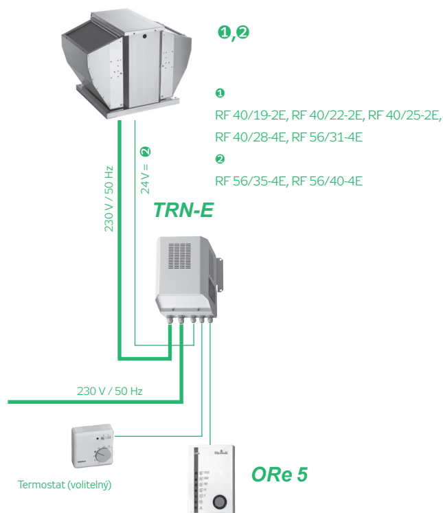
FIGURE 8 – FAN CONNECTION
