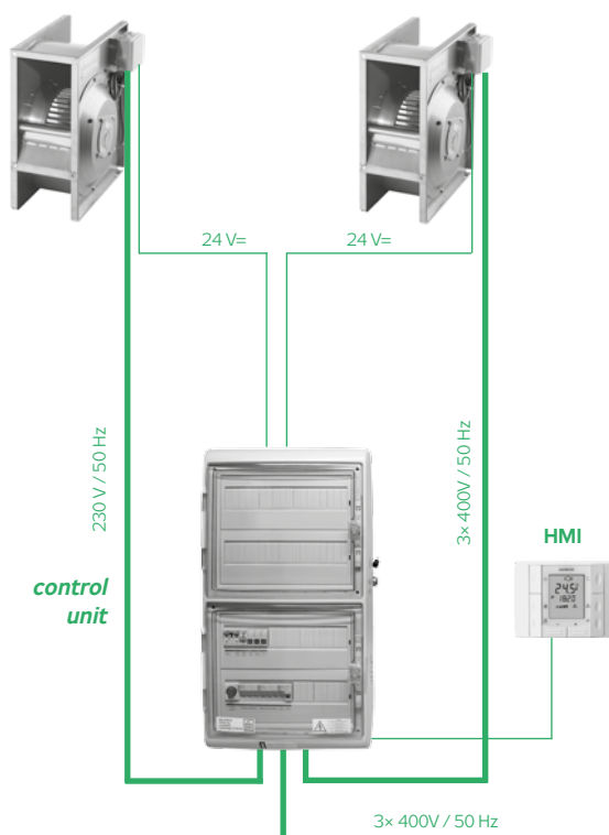
FIGURE 7 – FAN CONNECTION
