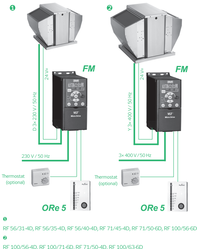
FIGURE 9 – FAN CONNECTION
