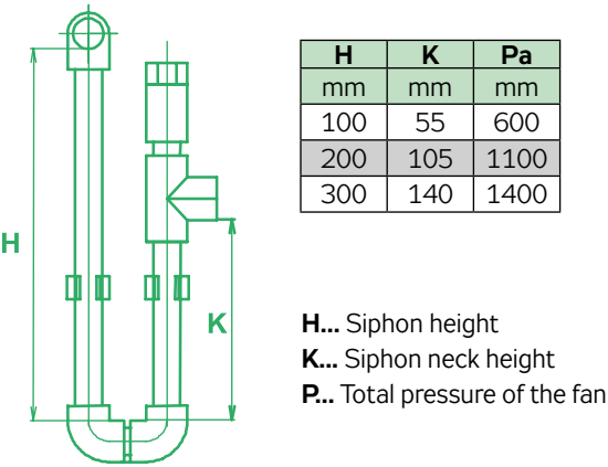
FIGURE 14 – CONDENSATE DRAINAGE
